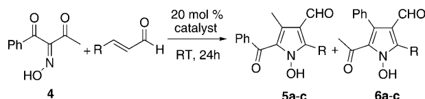
Scheme 2. Regioselectivity of the domino reaction.
